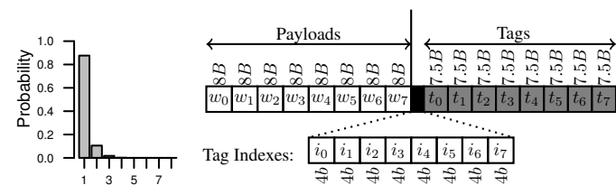
(a) Unique tags per DRAM transfer for gcc
