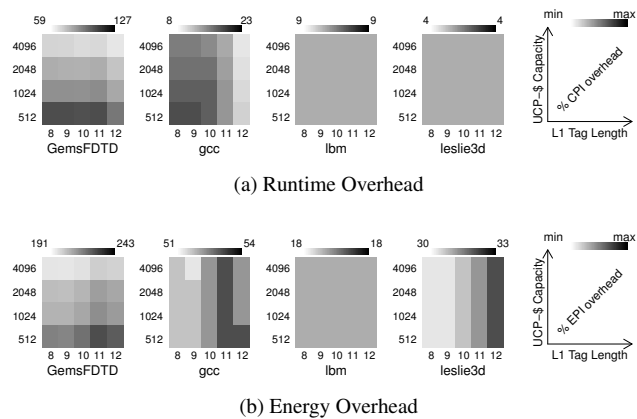
Figure 13: Impact of Tag Bits and UCP-$ Capacity
