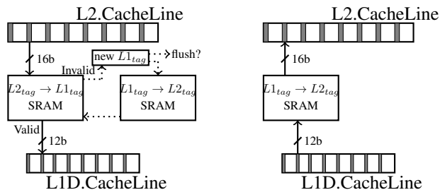
(a) L1 miss, L2 hit
